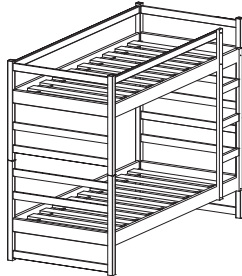
PEDRO K 53 Patrová postel JUNIOR 900x2000 s rošty 966x1650x2090
